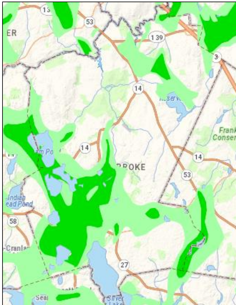
Figure 2-3. High and Medium Yield Aquifers in Pembroke
